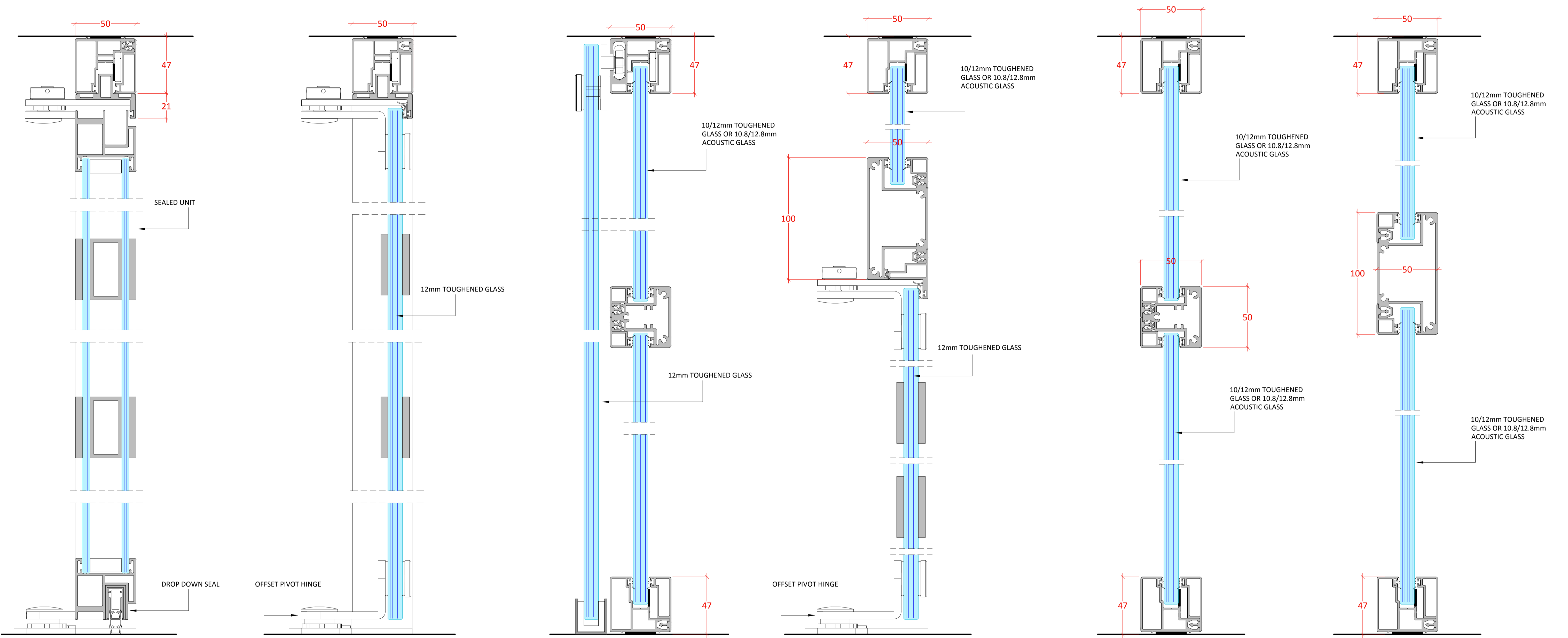
DOUBLE GLAZED FRAMED DOOR
