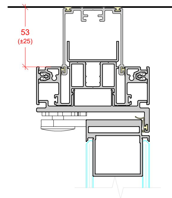
DEFLECTION HEAD ± 25mm
