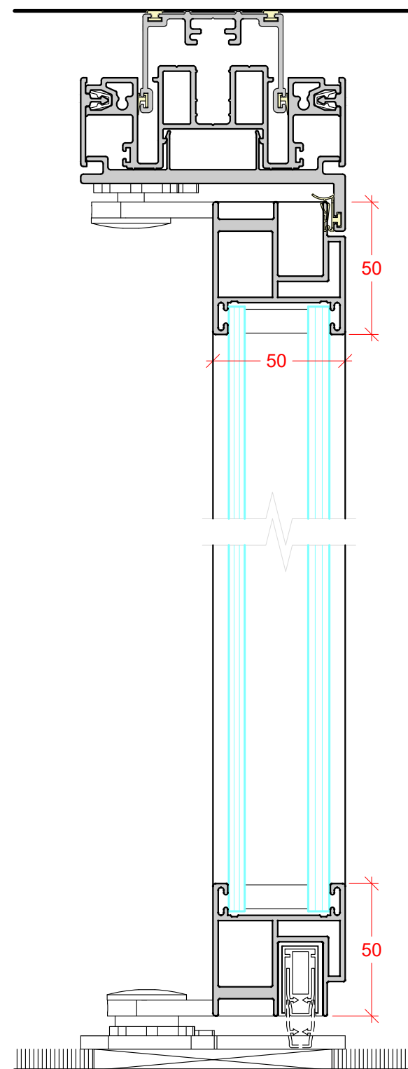
DOUBLE GLAZED PIVOT DOOR 36mm VACUUM GLASS FLOOR CLOSER IF REQUIRED
