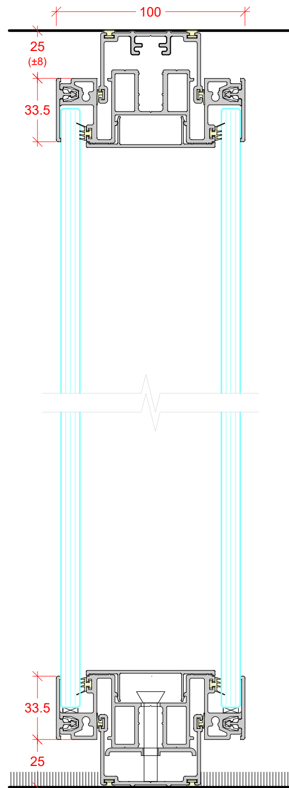
DOUBLE GLAZED 10mm, 10.8mm, 12mm & 12.8mm GLASS
