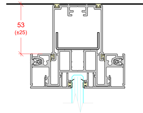
DEFLECTION HEAD ± 25mm
