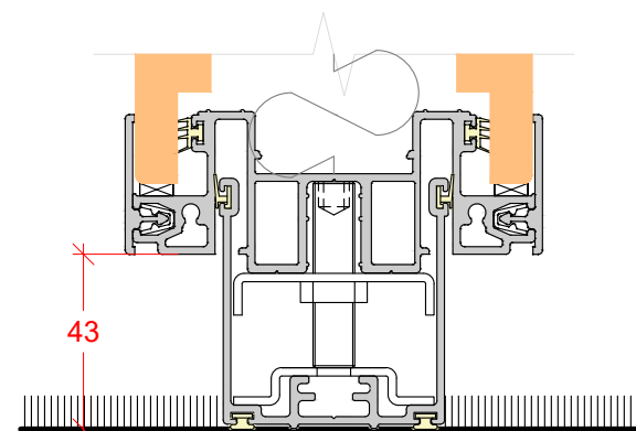
DEFLECTION HEAD ± 15mm
