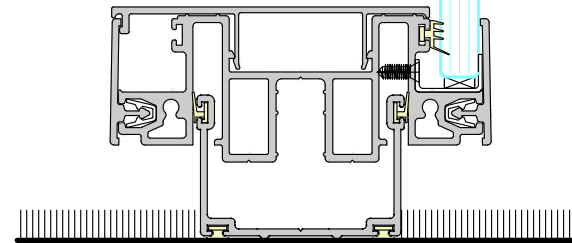
SINGLE GLAZED OFFSET GLAZING 10mm, 10.8mm, 12mm & 12.8mm GLASS
