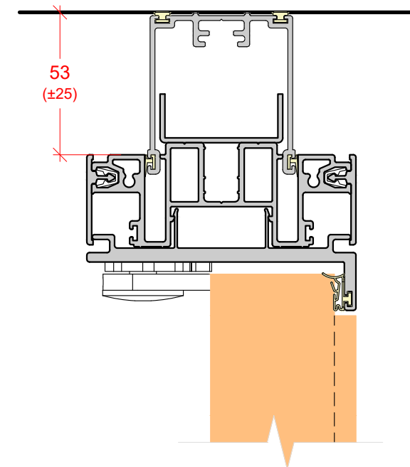
DEFLECTION HEAD ± 25mm
