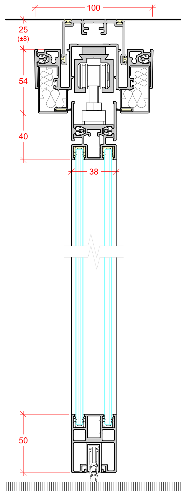
DOUBLE GLAZED SLIDING DOOR CLOSED POSITION 6mm + 6mm GLASS
