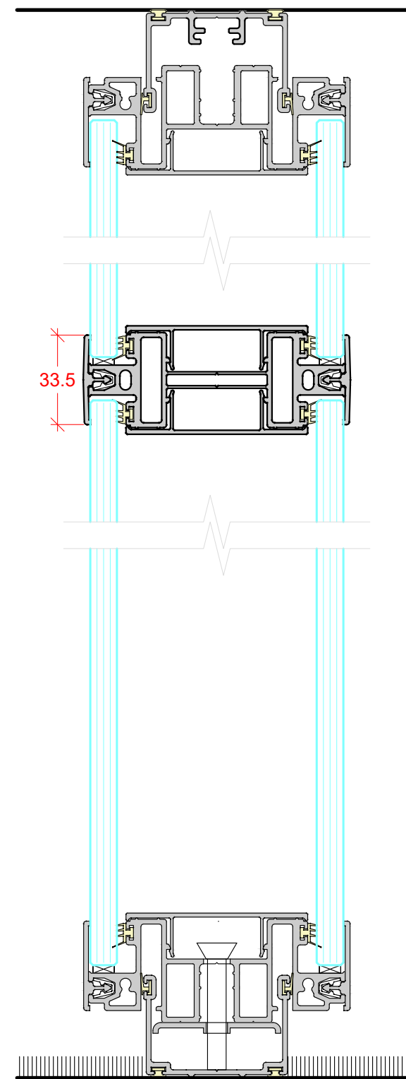
DOUBLE GLAZED OVER PANEL
