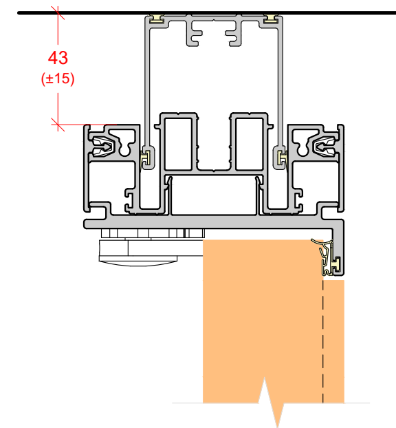
DEFLECTION HEAD ± 15mm
