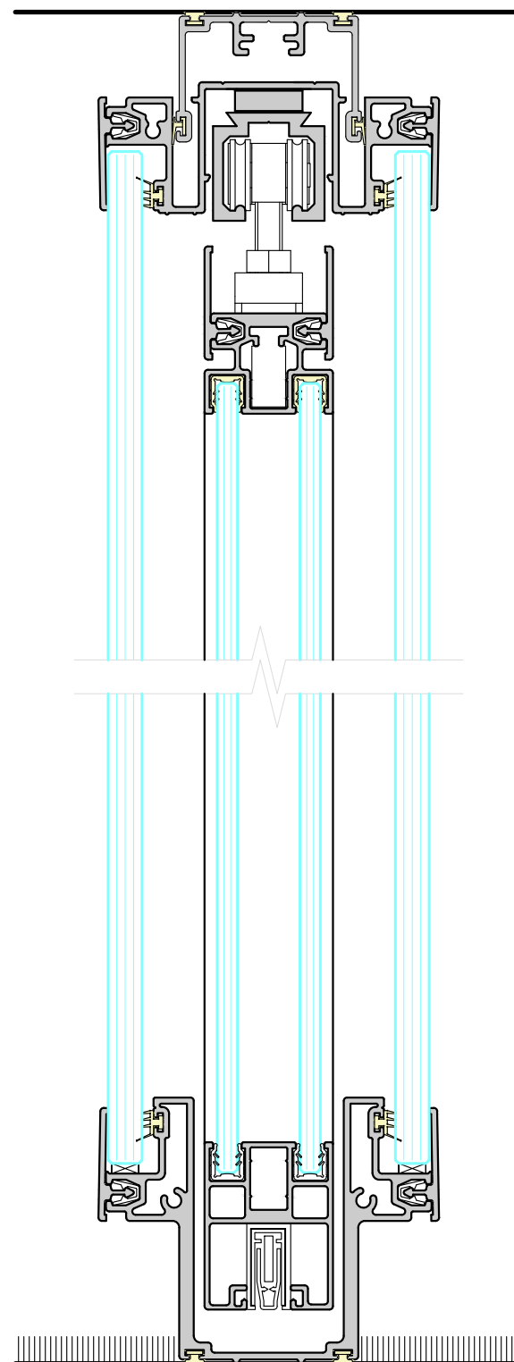
DOUBLE GLAZED SLIDING DOOR OPEN POSITION 6mm + 6mm GLASS
