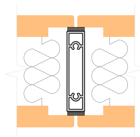
SOLID PANELS STRAIGHT JOINT
