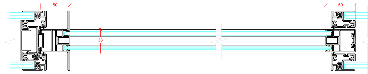
DOUBLE GLAZED SLIDING DOOR 6mm + 6mm GLASS
