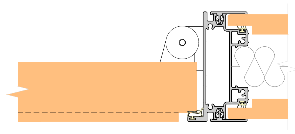
SOLID PANELS DOOR JUNCTION
