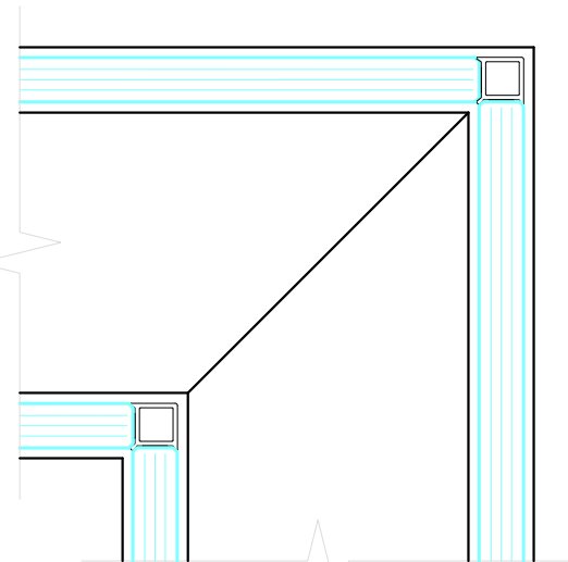
DOUBLE GLAZED CORNER JOINT POLYCARB CORNER JOINT
