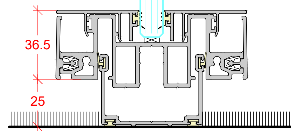
SINGLE GLAZED CENTRAL GLAZING 10mm, 10.8mm, 12mm & 12.8mm GLASS
