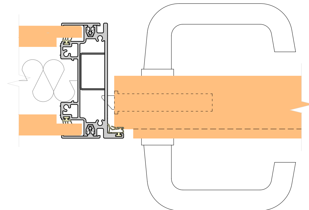
SOLID PANELS DOOR JUNCTION
