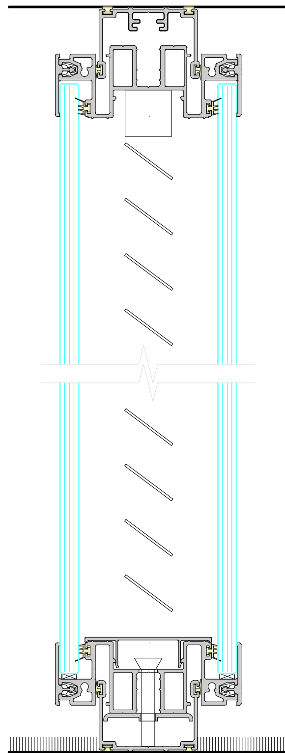
DOUBLE GLAZED INTEGRATED BLIND
