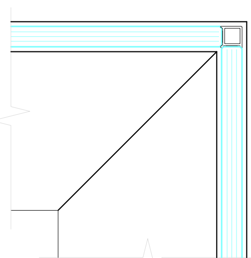
SINGLE GLAZED CORNER JOINT OFFSET GLAZING POLYCARB CORNER JOINT
