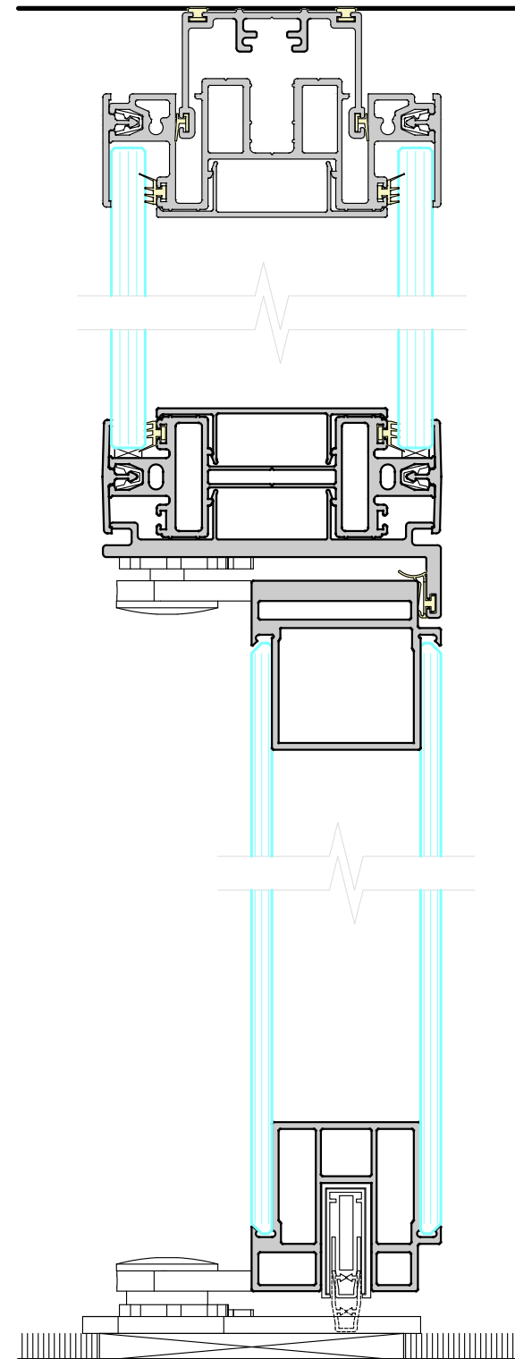
PIVOT DOOR OVER PANEL FLOOR CLOSER IF REQUIRED
