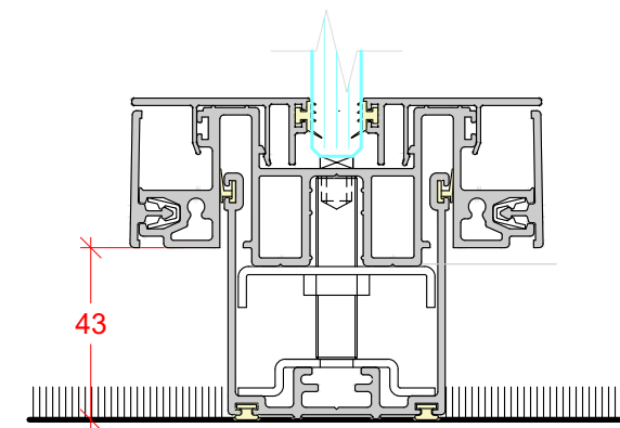
DEFLECTION HEAD ± 15mm
