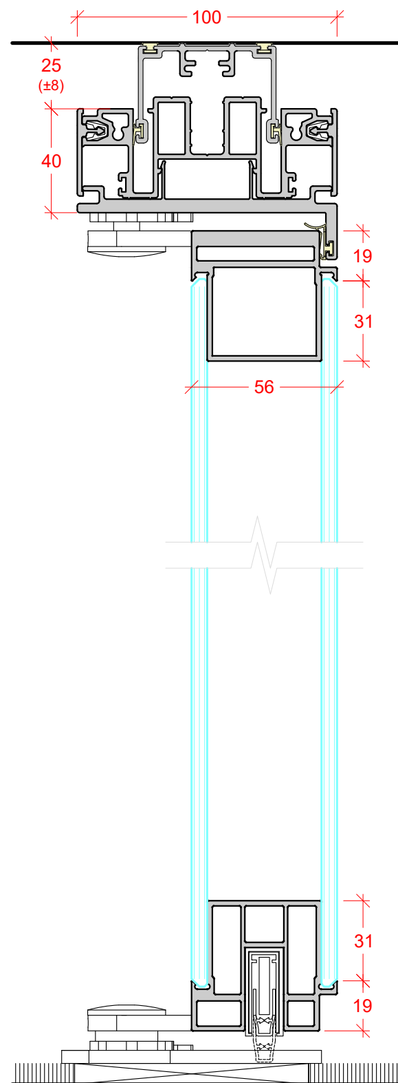
DOUBLE GLAZED PIVOT DOOR 6mm + 6mm GLASS FLOOR CLOSER IF REQUIRED
