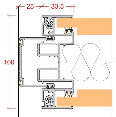
SOLID PANELS WALL ABUTMENT
