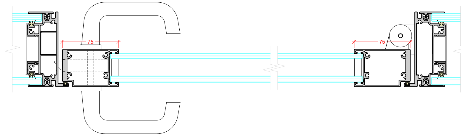
DOUBLE GLAZED PIVOT DOOR 36mm VACUUM GLASS
