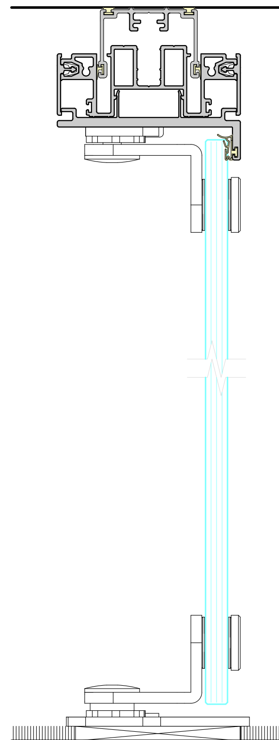
SINGLE GLAZED PIVOT DOOR 10mm, 12mm GLASS FLOOR CLOSER IF REQUIRED
