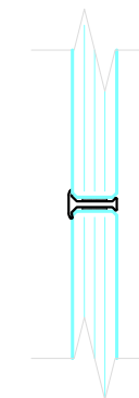
GLASS STRAIGHT JOINT ALUMINIUM STRAIGHT JOINING STRIP
