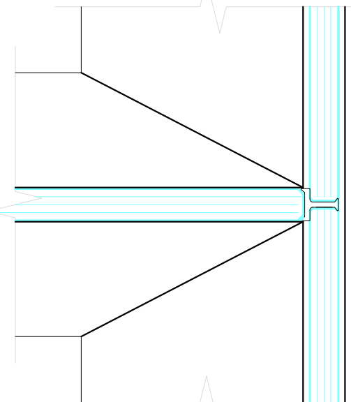
SINGLE GLAZED 3 WAY JUNCTION OFFSET / CENTRAL GLAZING POLYCARB 3 WAY JUNCTION
