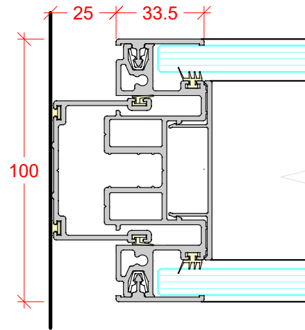
WALL ABUTMENT
