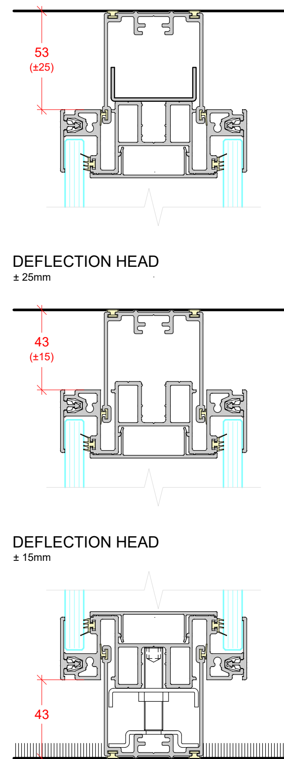
DOUBLE GLAZED 43mm BASE
