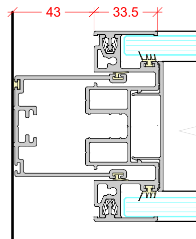
WALL ABUTMENT
