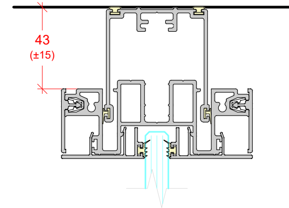
DEFLECTION HEAD ± 15mm
