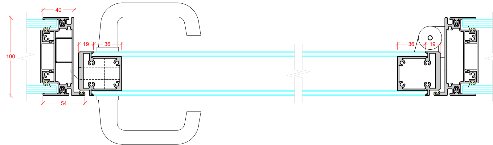
DOUBLE GLAZED PIVOT DOOR 6mm + 6mm GLASS
