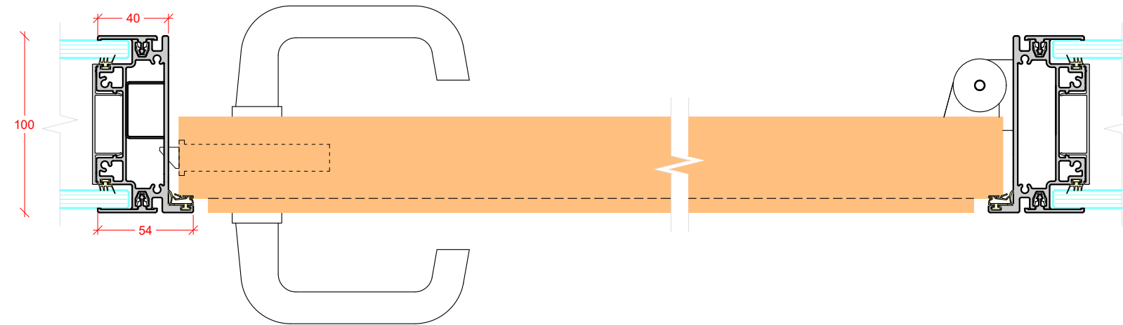
SOLID PIVOT DOOR 44mm & 54mm LEAF
