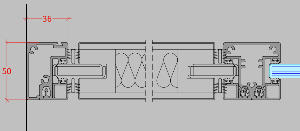
WALL ABUTMENT TO SOLID PANEL TO BROOKLYN SECTION 10mm toughened glass
