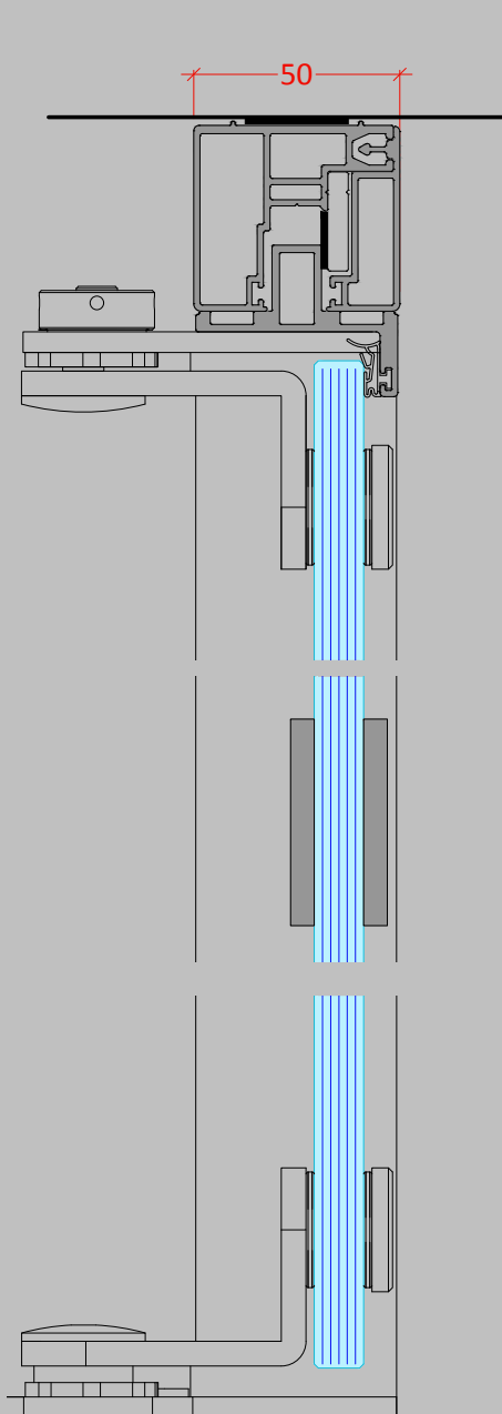
SINGLE GLAZED OFFSET PIVOT DOOR 12mm toughened glass
