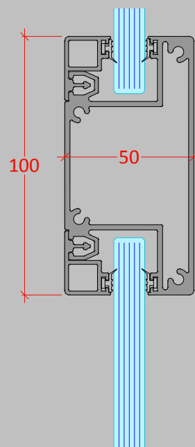
BROOKLYN SECTION 100mm x 50mm
