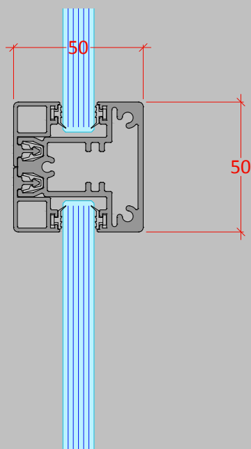
BROOKLYN SECTION 50mm x 50mm
