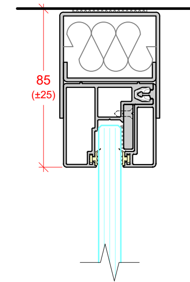
SINGLE GLAZED DEFLECTION HEAD \pm 25\text{mm}
