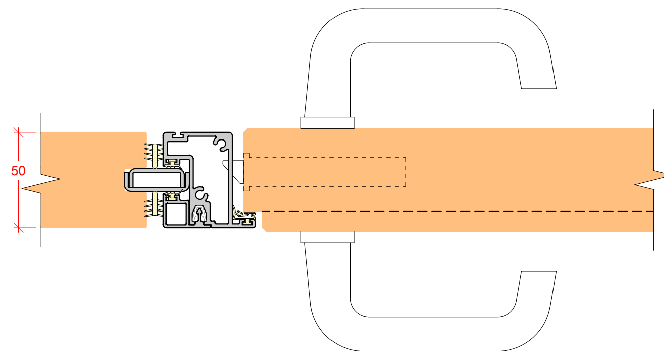
SOLID PANEL DOOR JUNCTION
