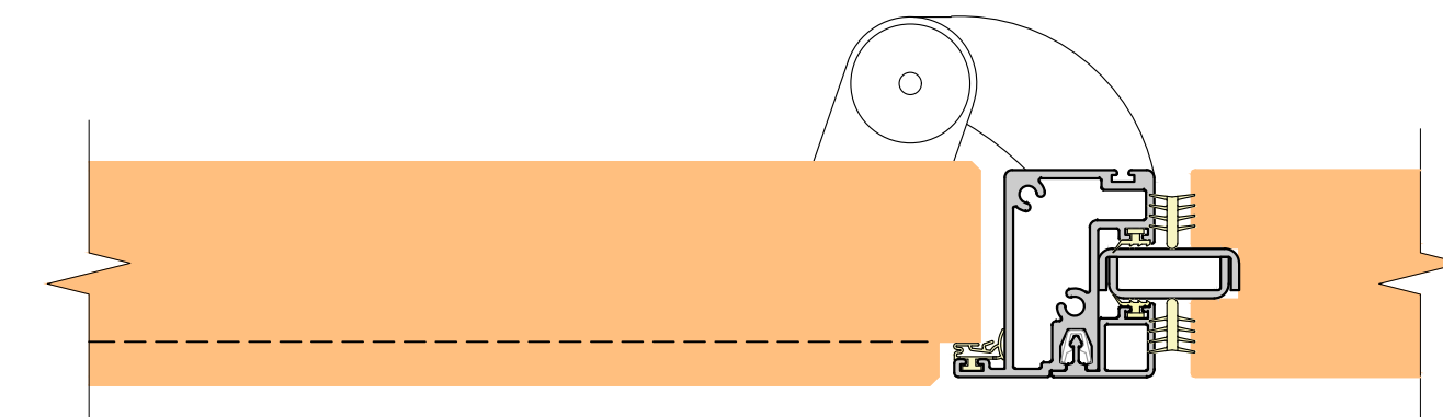
SOLID PANEL DOOR JUNCTION
