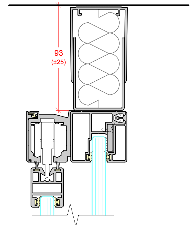
DEFLECTION HEAD ± 25mm
