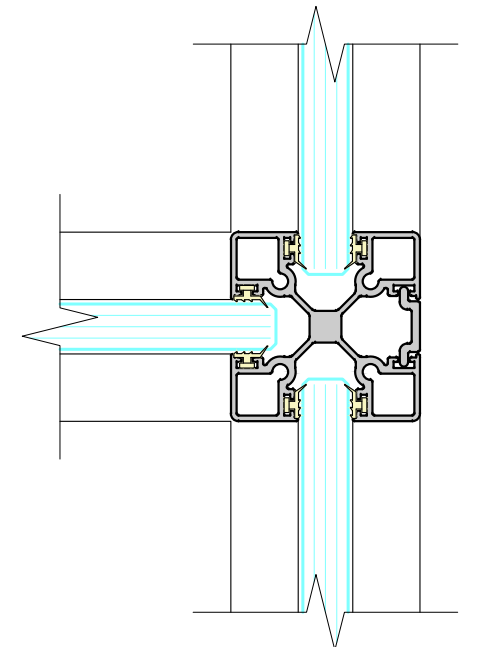
GLASS 3 WAY JUNCTION JUNCTION POST
