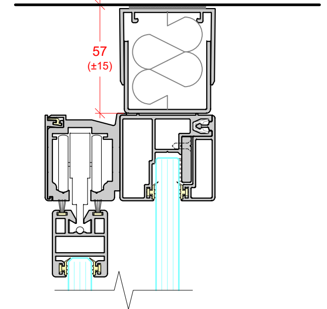
DEFLECTION HEAD ± 15mm
