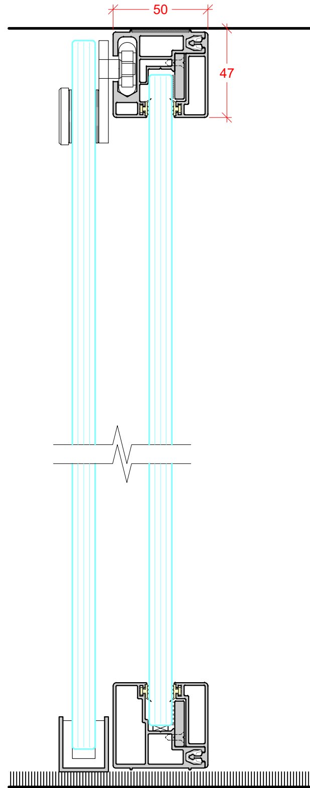
SINGLE GLAZED SLIDING DOOR FRAMELESS DOOR 10mm, 12mm GLASS
