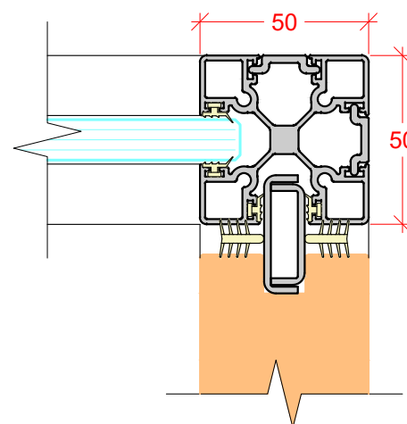
SOLID PANEL / GLAZING CORNER JUNCTION
