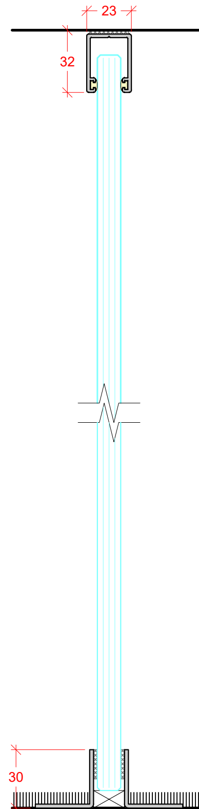
SINGLE GLAZED SLIM 10mm, 10.8mm, 12mm & 12.8mm GLASS
