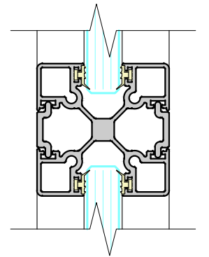
GLASS STRAIGHT JOINT JUNCTION POST
