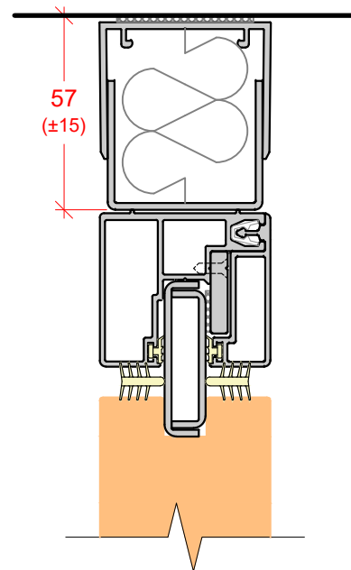
DEFLECTION HEAD ±15mm
