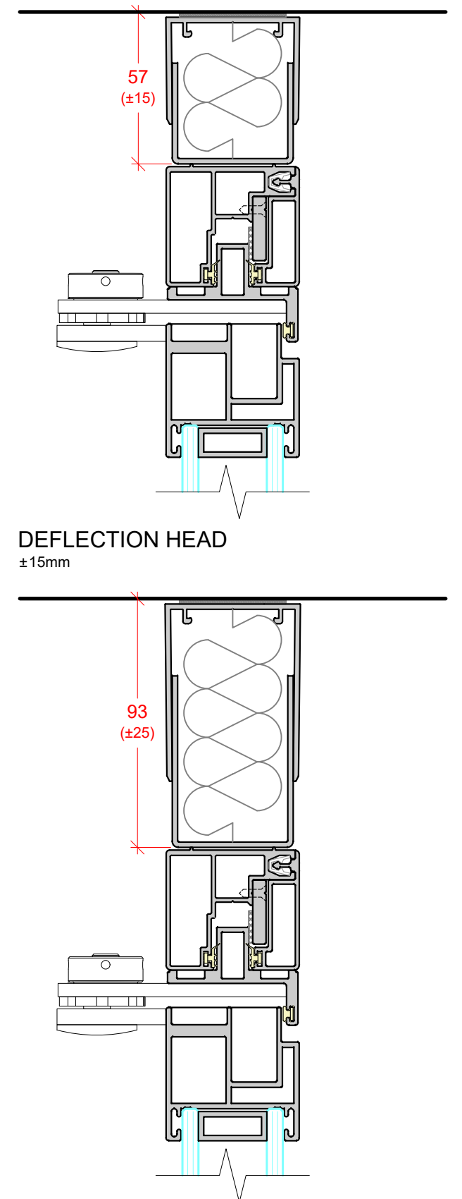
DEFLECTION HEAD ±25mm
