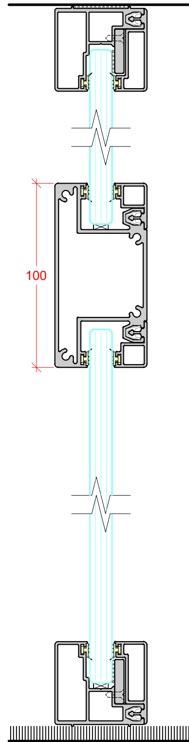
SINGLE GLAZED OVER PANEL
