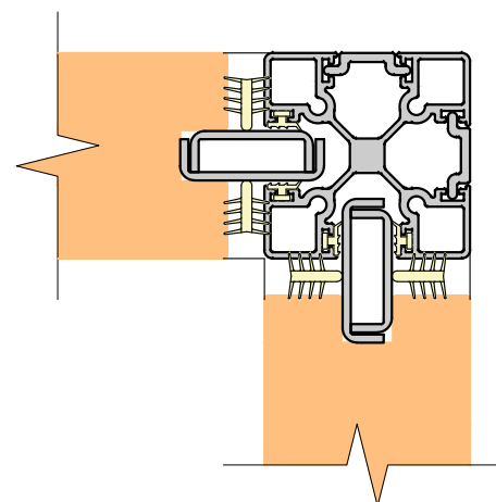
SOLID PANEL CORNER JUNCTION
