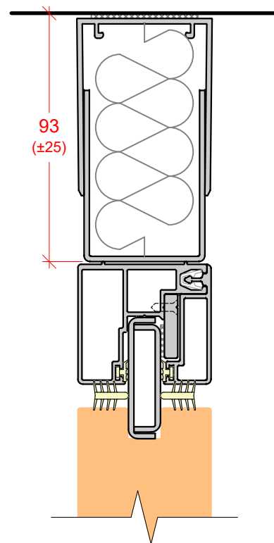
DEFLECTION HEAD ±25mm
