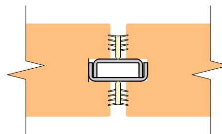
SOLID PANEL STRAIGHT JUNCTION
