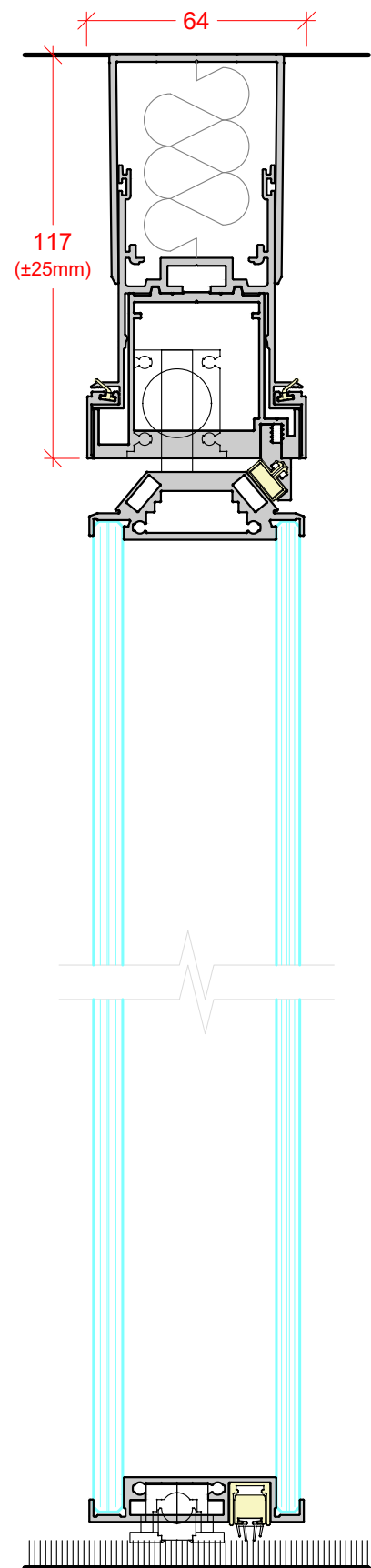
DOUBLE GLAZED PIVOT DOOR 8mm + 6mm ACOUSTIC LAMINATED GLASS
