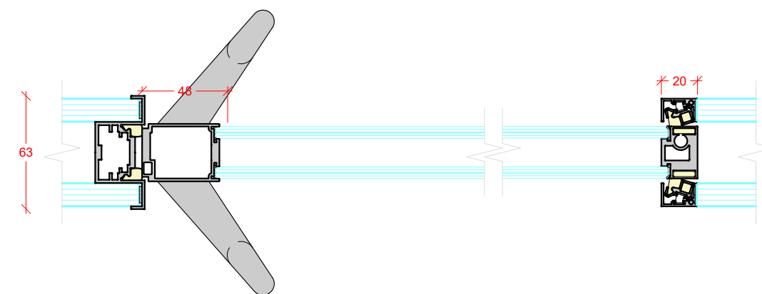
DOUBLE GLAZED SLIDING DOOR 6mm + 6mm ACOUSTIC LAMINATED GLASS CUSTOM PULL HANDLE
