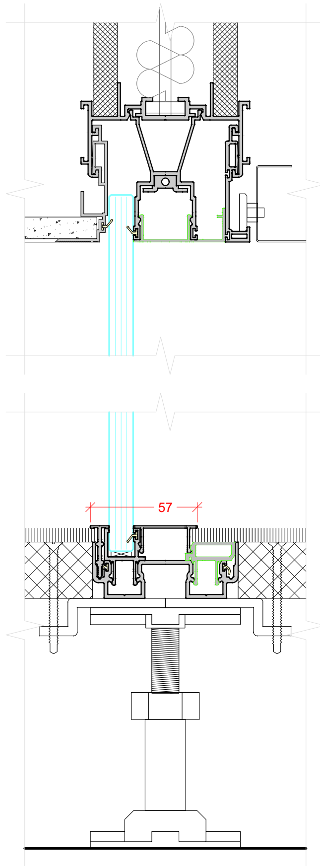
SINGLE GLAZED OFFSET GLAZING 10mm, 10.8mm, 12mm & 12.8mm GLASS
