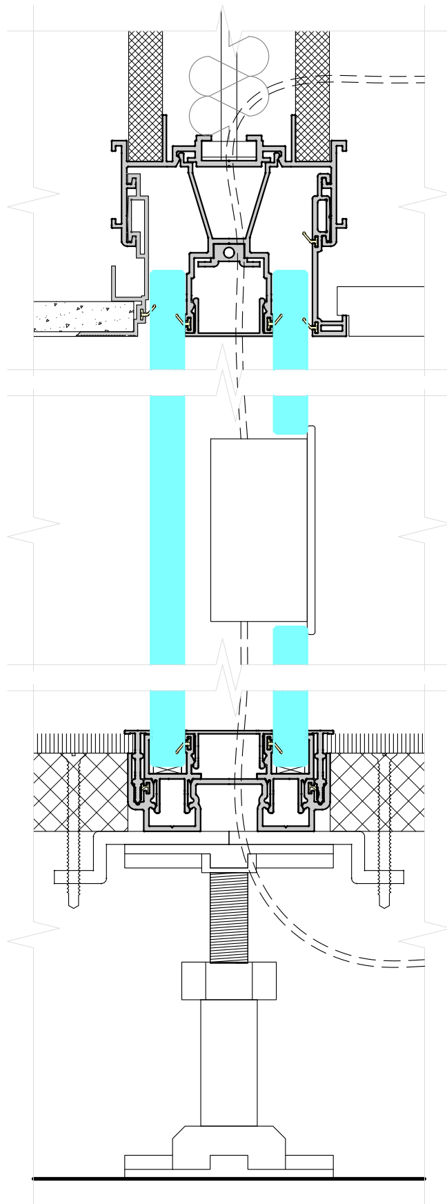
TECH PANEL BACK PAINTED GLASS
