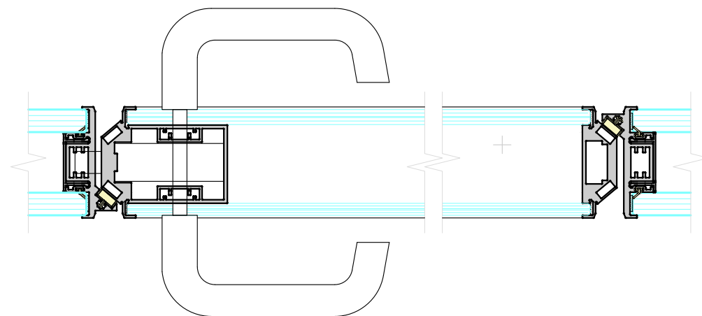
DOUBLE GLAZED PIVOT DOOR 8mm + 6mm ACOUSTIC LAMINATED GLASS / LATCH CUSTOM HANDEL
