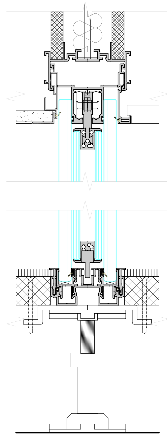
DOUBLE GLAZED SLIDING DOOR OPEN POSITION 6mm + 6mm ACOUSTIC LAMINATED GLASS
