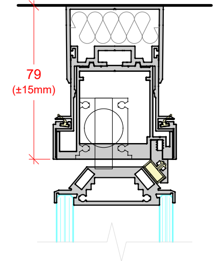
DEFLECTION HEAD ± 15mm
