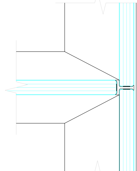
SINGLE GLAZED 3 WAY JUNCTION OFFSET / CENTRAL GLAZING POLYCARB 3 WAY JUNCTION
