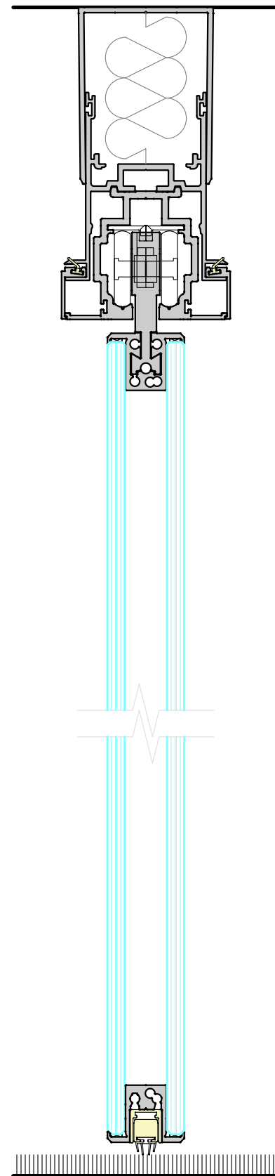
DOUBLE GLAZED SLIDING DOOR CLOSED POSITION 6mm + 6mm ACOUSTIC LAMINATED GLASS
