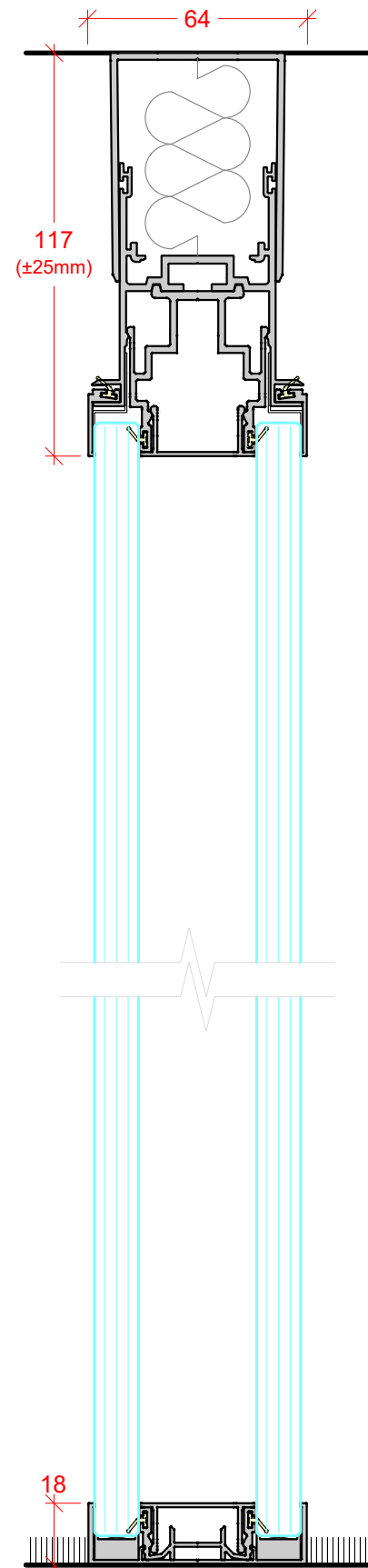
DOUBLE GLAZED 10mm, 10.8mm, 12mm & 12.8mm GLASS
