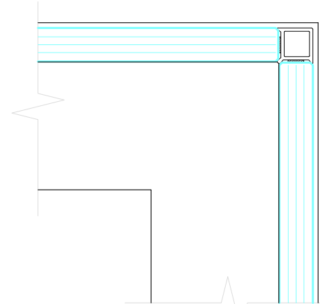
SINGLE GLAZED CORNER JOINT OFFSET GLAZING POLYCARB CORNER JOINT
