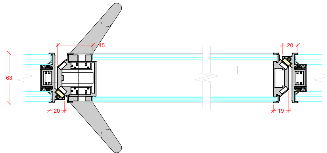
DOUBLE GLAZED PIVOT DOOR 8mm + 6mm ACOUSTIC LAMINATED GLASS WITH OLIVE CATCH
