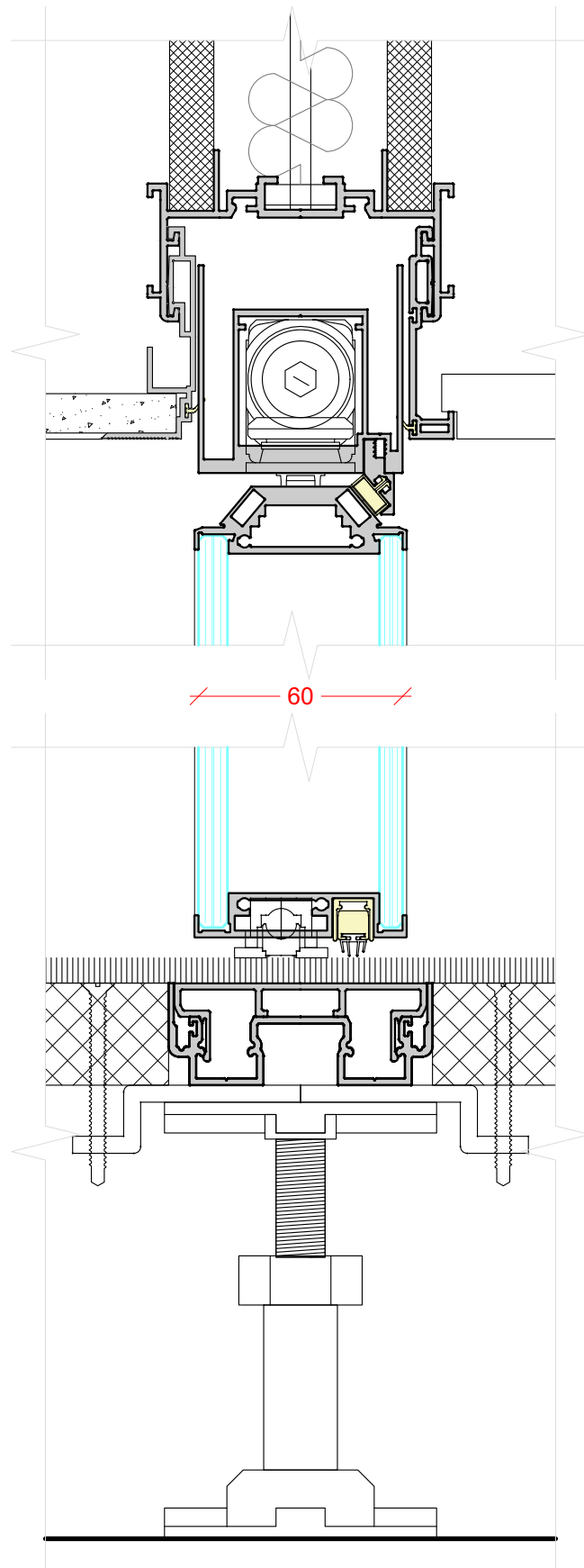
DOUBLE GLAZED PIVOT DOOR 8mm + 6mm ACOUSTIC LAMINATED GLASS
