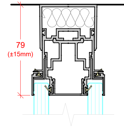
DEFLECTION HEAD ± 15mm
