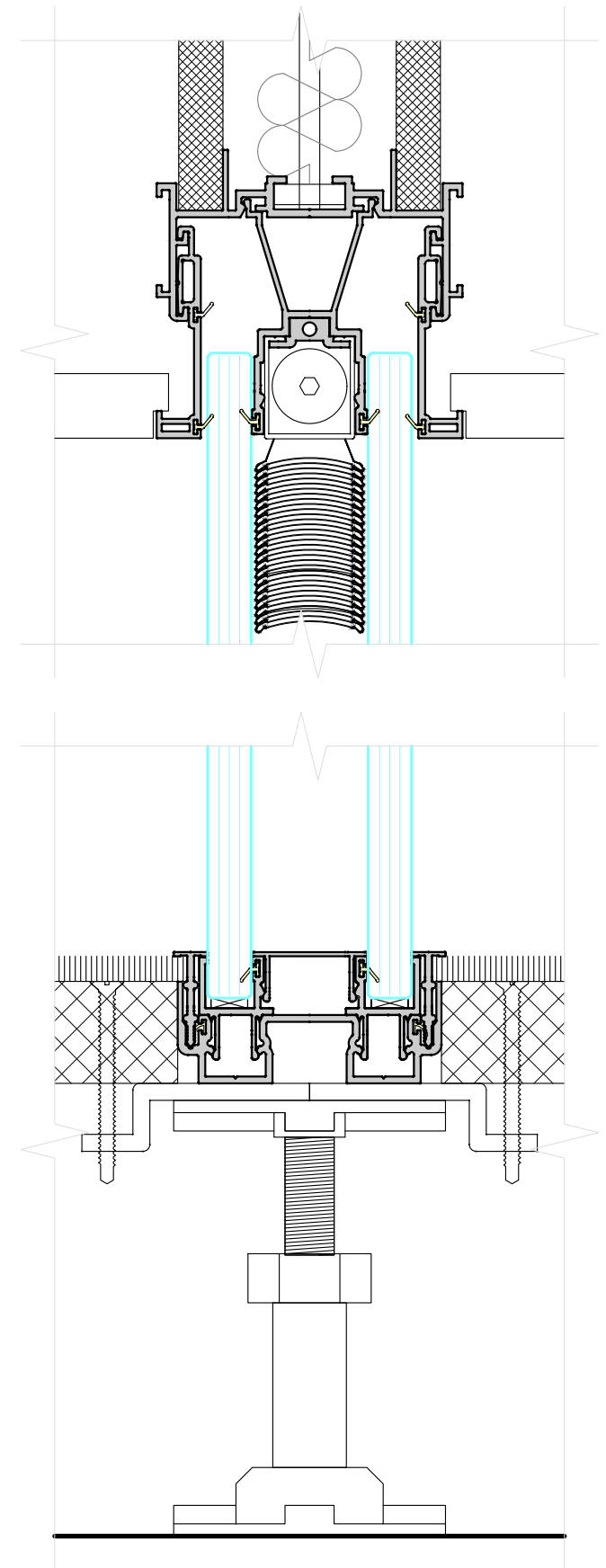
DOUBLE GLAZED INTEGRATED BLIND
