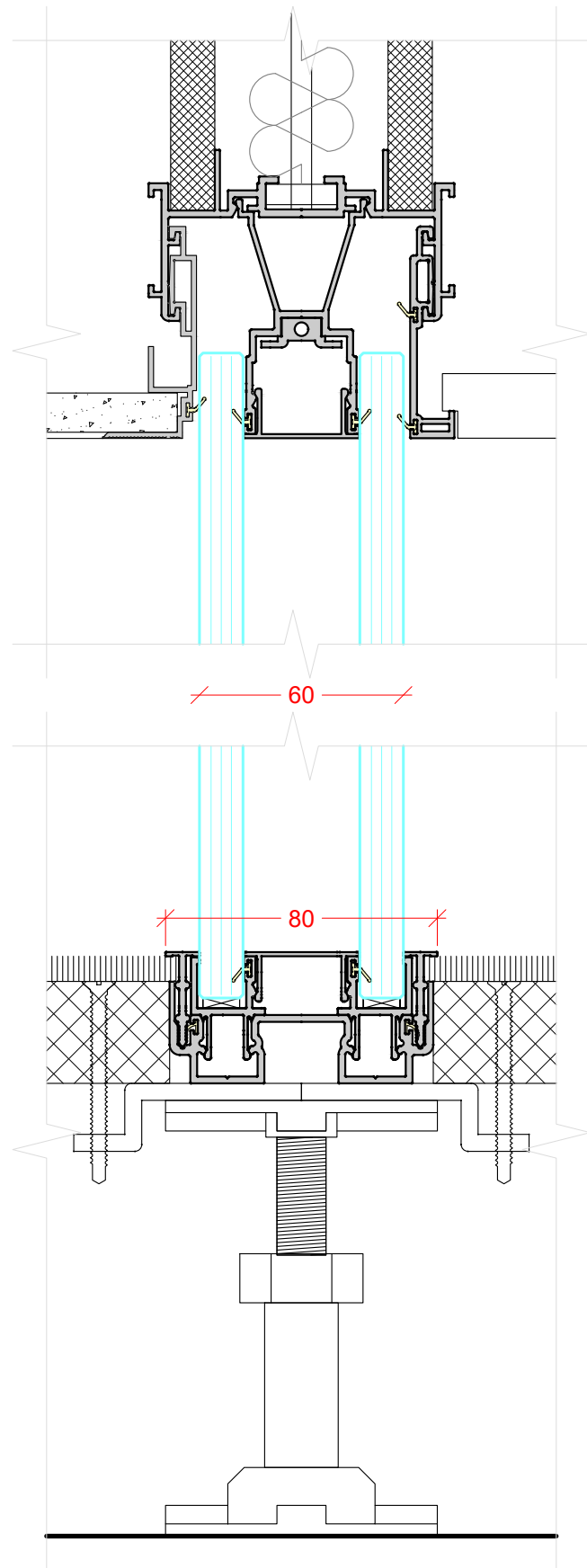
DOUBLE GLAZED 10mm, 10.8mm, 12mm & 12.8mm GLASS
