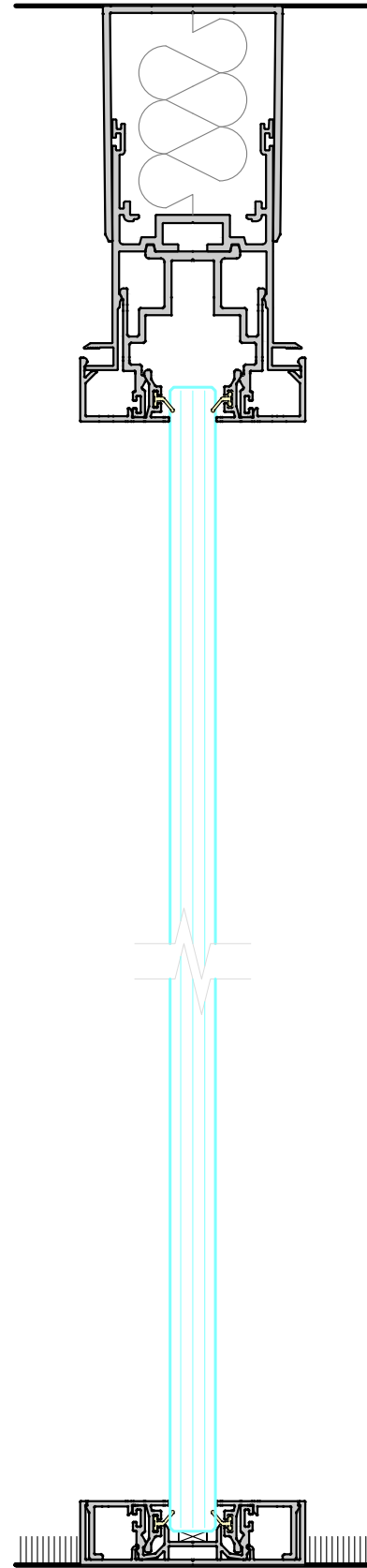
SINGLE GLAZED CENTRAL GLAZING 10mm, 10.8mm, 12mm & 12.8mm GLASS
