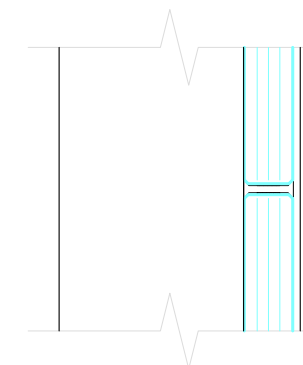
SINGLE GLAZED STRAIGHT JOINT OFFSET GLAZING POLYCARB STRAIGHT JOINT
