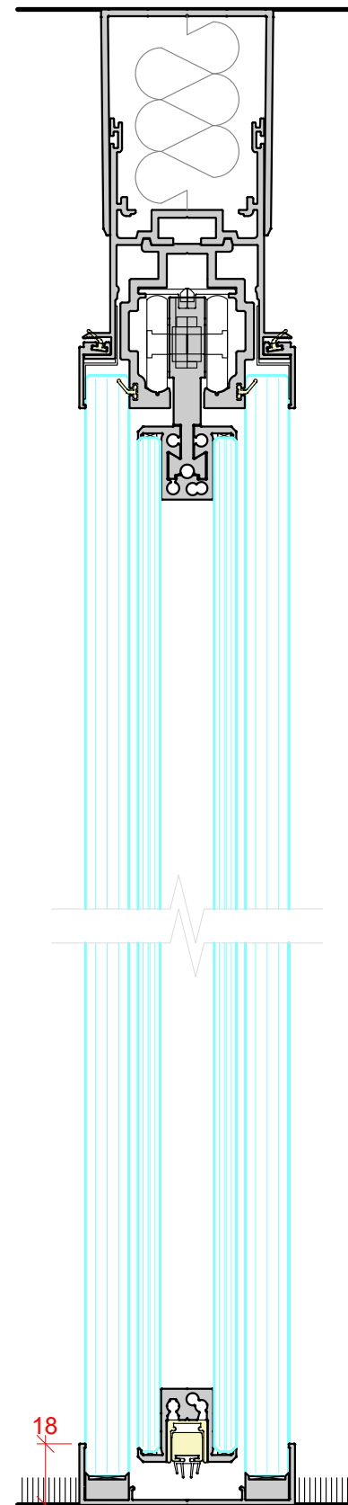
DOUBLE GLAZED SLIDING DOOR OPEN POSITION 6mm + 6mm ACOUSTIC LAMINATED GLASS
