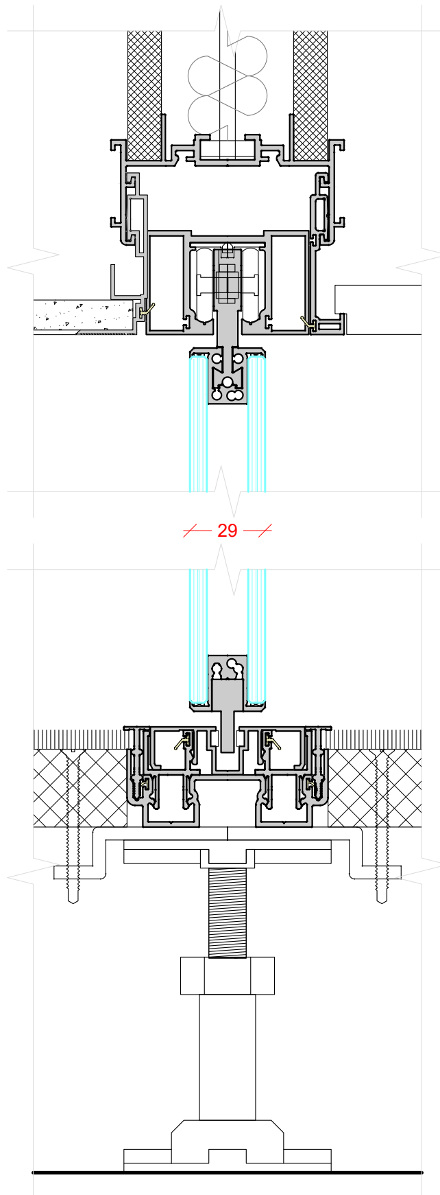
DOUBLE GLAZED SLIDING DOOR CLOSED POSITION 6mm + 6mm ACOUSTIC LAMINATED GLASS
