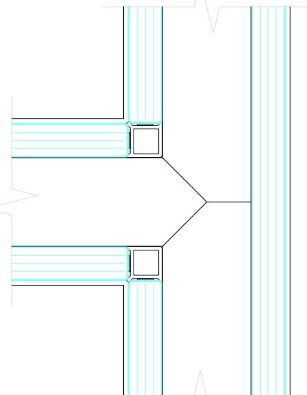
DOUBLE GLAZED 3 WAY JUNCTION POLYCARB 3 WAY JUNCTION
