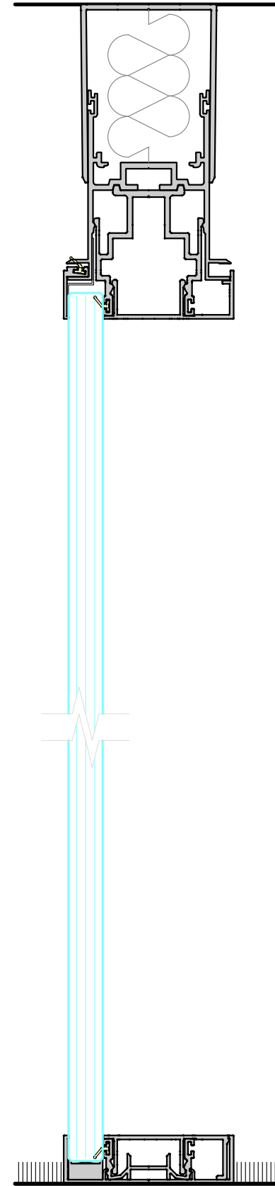
SINGLE GLAZED OFFSET GLAZING 10mm, 10.8mm, 12mm & 12.8mm GLASS
