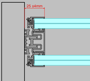
WALL ABUTMENT Deflection - \pm 5\text{mm}
