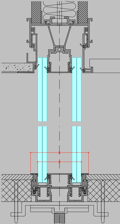
DOUBLE GLAZED PARTITION 12.8 mm acoustic laminate glass Ceiling tile option and plasterboard option
