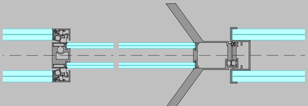
DOUBLE GLAZED SLIDING DOOR Sliding door with magnetic gaskets
