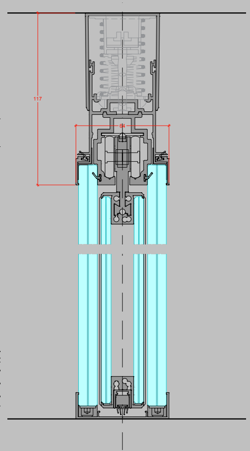
DOUBLE GLAZED SLIDING DOOR IN DOUBLE GLAZED PARTITION Non - Integrated
