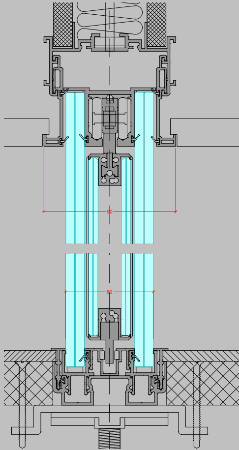
DOUBLE GLAZED SLIDING DOOR IN DOUBLE GLAZED PARTITION Integrated
